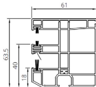
Guida (PVC) singola + MKT* R0003
